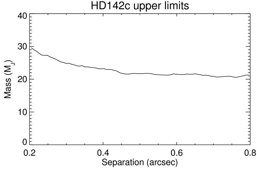
Figure 5.13: Upper limits of the mass estimated from IFS detection curve. The cancellation has been taken into account during the calculation of detection limits. The models used for the conversion luminosity contrast/mass are the AMES-COND.
