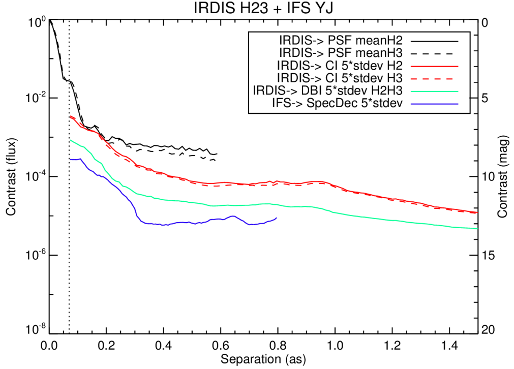
Figure 4.1: 5\sigma residual noise levels, without ADI reduction, for the two science modules of SPHERE, IRDIS and IFS, in IRDIFS mode. The curves refer to the dataset described in Table 6.1, where I injected the synthetic planets. The vertical dotted line represents the radius of the coronagraph, i.e., the zone where the detectors are blind. The mean azimuthal profile of the off-axis PSF (black), the coronagraphic profile (red) are shown for the two IRDIS channels H2 (continuous line) and H3 (dashed line). The contrast results after the SDI reduction (green) and SD reduction for IFS (blue) are shown.
