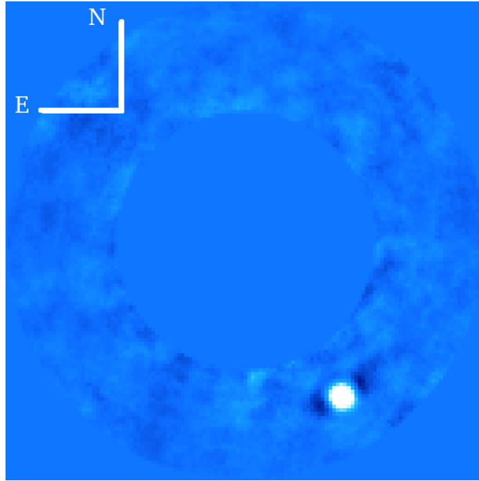
Figure 4.11: One of the IFS channels showing \beta Pic b. The reduction has been made with KLIP routine.
