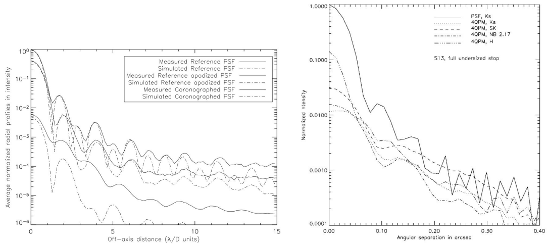
Figure 1.11: Light suppression achievable with the Lyot (left) and the 4QPM (right) coronagraphs of SPHERE. Images taken from Guerri et al. (2009) and Boccaletti et al. (2004). In the first case, simulations and laboratory results are shown, in the second only measured laboratory results are shown.
