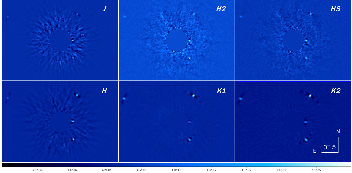
Figure 6.1: IRDIS images for several filters with the four planets around HR 8799 obtained with the rADI, T-LOCI and KLIP pipelines. The color scale is the same for all images.
