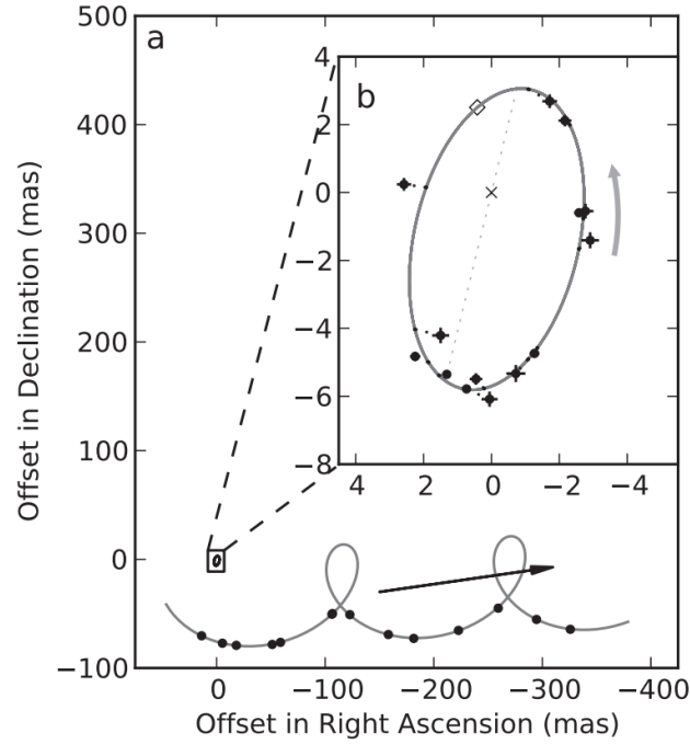
Figure 1.6: Example of astrometry detection of a low mass companion to an ultracool dwarf (Sahlmann et al. 2013).
