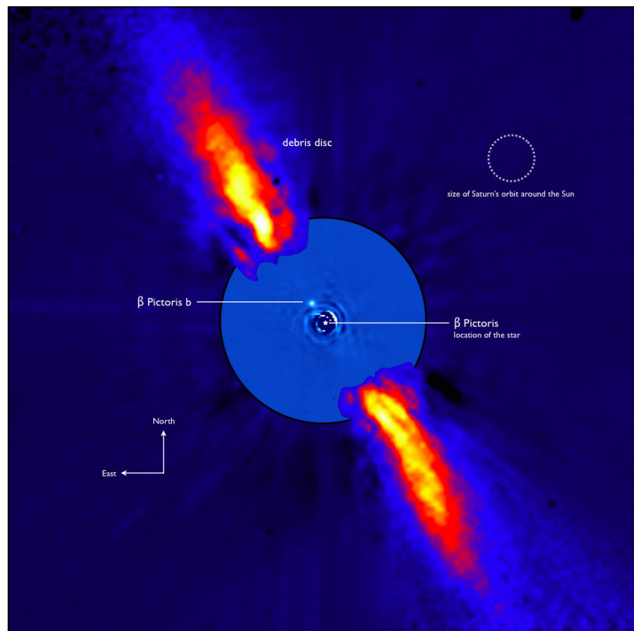
Figure 1.20: Image of \beta Pic, showing the planet and the debris disk around it (Lagrange et al. 2009).
