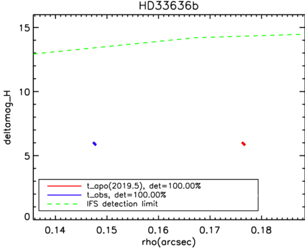
Figure 5.6: Contrast in H band of the stellar companion HD 33636 B. In the lower part of the plot are shown the probability of detection. This object, for its brightness, is always detectable with SPHERE.
