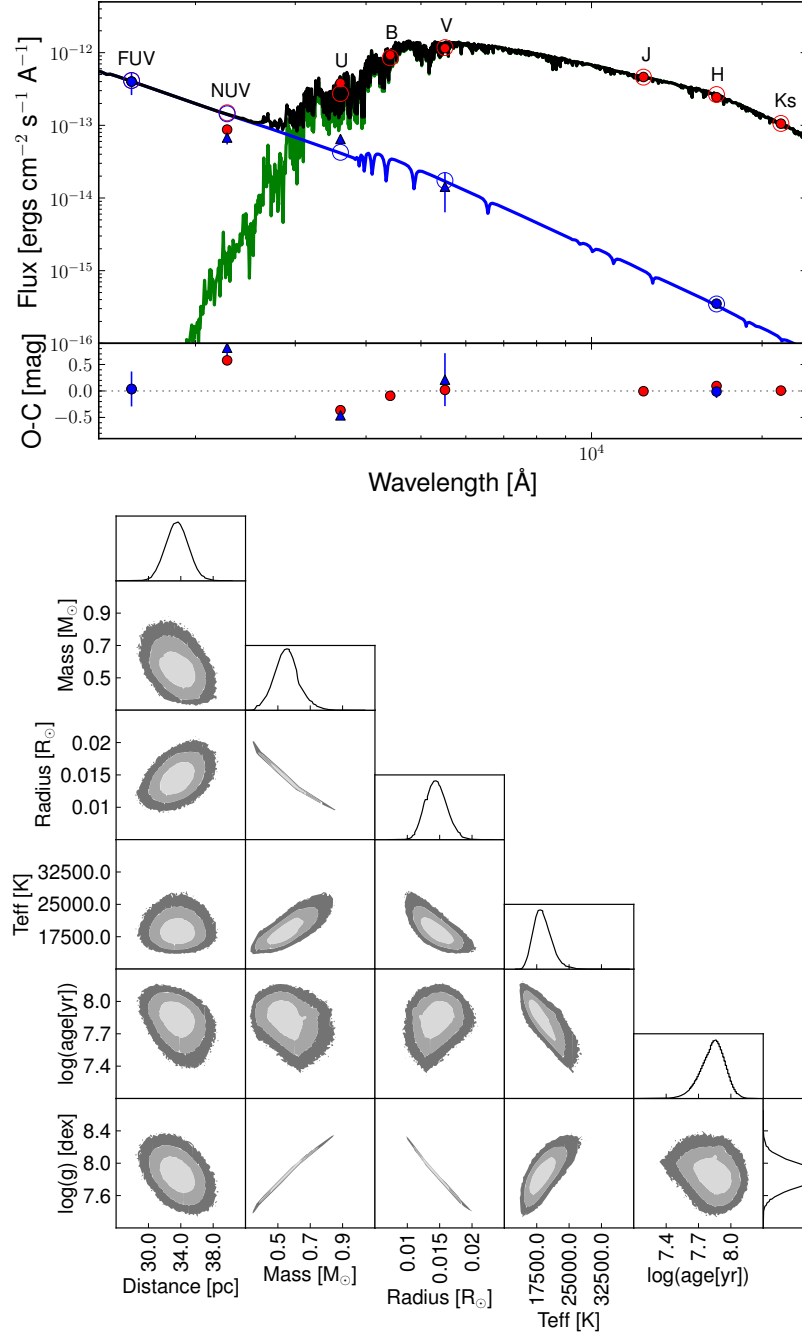
Figure 3.6: Top: Observed magnitudes of the system plotted over the synthetic spectra. Blue points are those taken in consideration during the SED fitting of the WD. Triangle-shaped ones are not considered during the PASTIS integration. Values of the magnitudes of the integrated system are represented in red and the SED in black. The primary star SED is represented in green. Bottom: Two parameters joint posterior distributions for HD 8049 B. The 68.3%, 95.5% and 99.7% confidence regions are denoted by light gray, dark gray and black areas, respectively. Single PDF of each combination is shown along the sides.
