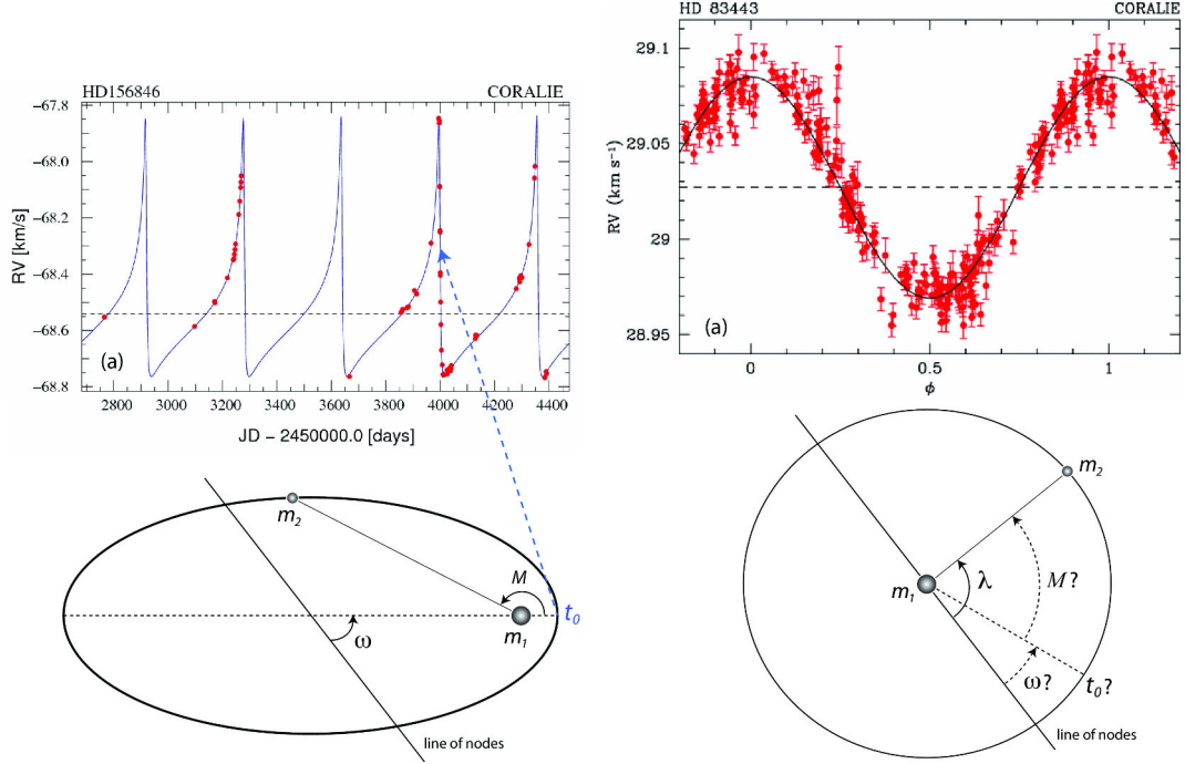
Figure 1.2: High eccentricity planet (left panel) and low (right panel) RV plots from Murray & Correia (2011).
