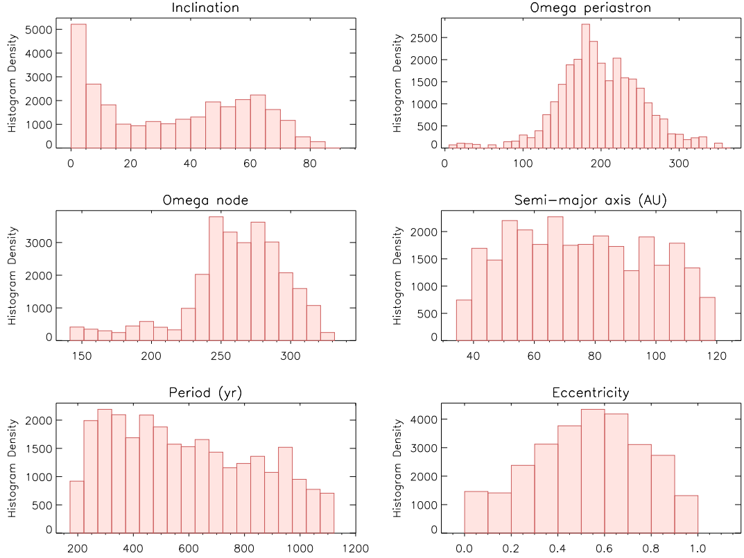
Figure 3.10: Histograms of orbital parameters derived with a Monte Carlo simulation following the example of Desidera et al. (2011).
