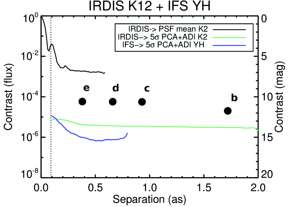
Figure 6.3: Contrast curves for the IRDIFS_EXT dataset. The 5\sigma contrast for the two instruments are plotted as a function of the angular separation. Planets around HR 8799 are also shown as photometric K2 points, the error bars are inside the dimension of the dots. The dotted vertical line indicates the coronagraph IWA.
