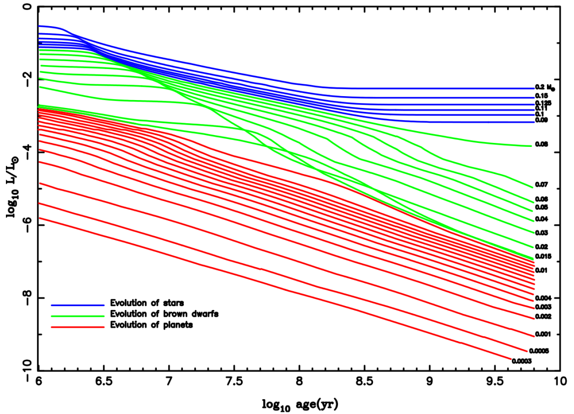
Figure 1.29: Figure taken from Burrows et al. (1997). Evolution of the luminosity of sub-stellar objects in function of their age. The distinction of the planetary/brown dwarf/stellar regime is represented by red/green/blue colors. The mass is labeled in the right edge of each evolutionary track.
