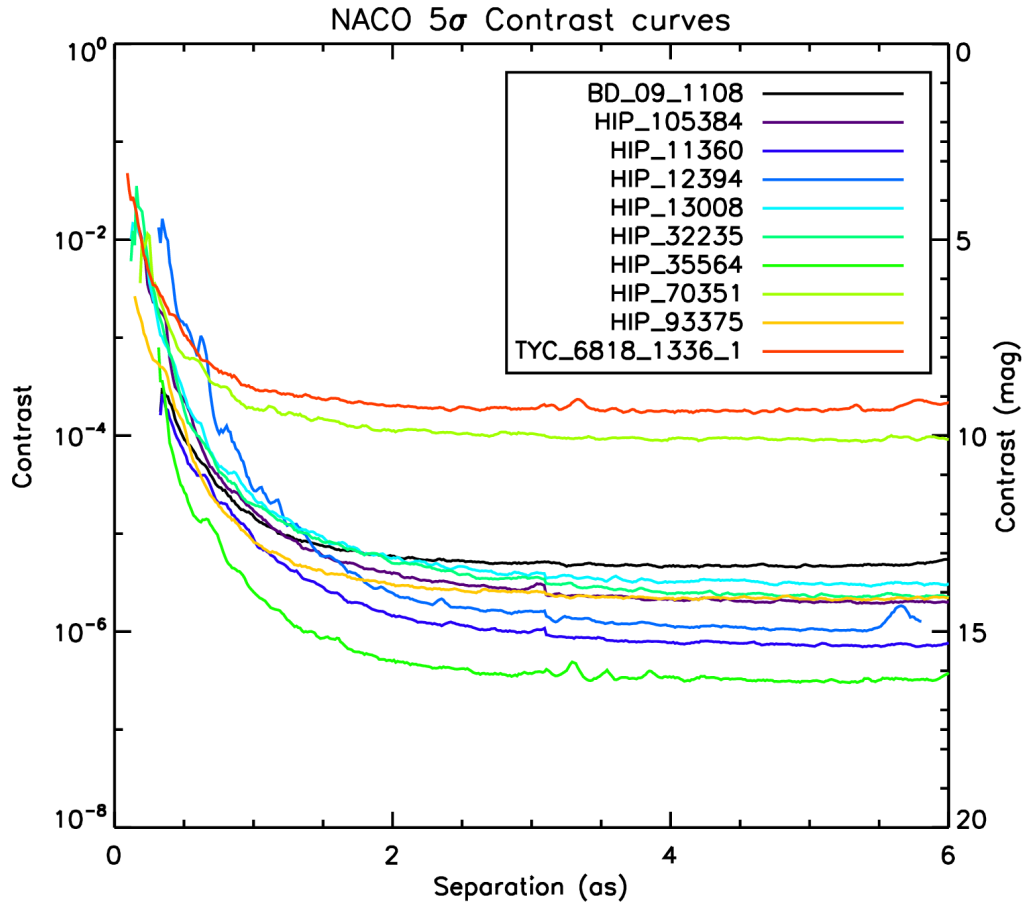
Figure 2.1: Some examples of contrast curves, including the worst and the best, of deep ADI observations with NACO. The names of each targets are labeled in the legend. Contrast values for NACO targets kindly given by A. Vigan.
