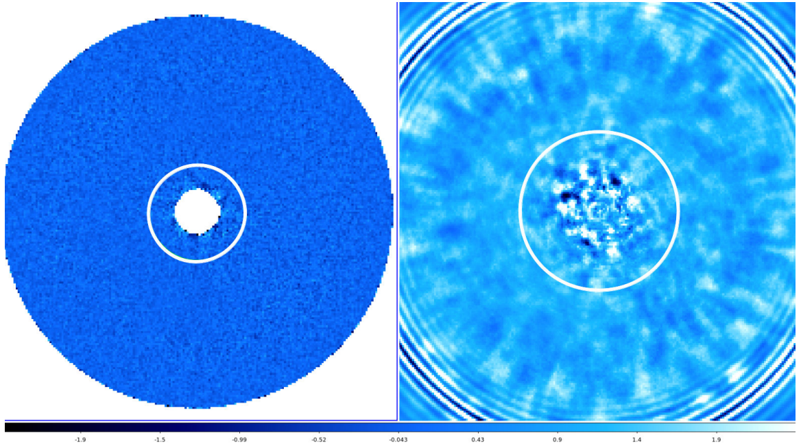
Figure 5.11: SDI+ADI reduction of SPHERE/IRDIS H2H3 channels for the object HD 142 A (left), and ADI reduction of SPHERE/IFS datacube (right). For IFS the median of the channels is shown. In the detectors no point above 5\sigma is detected. The white circle indicates a distance of 0''.3 from the center, where the planet is expected to be found.
