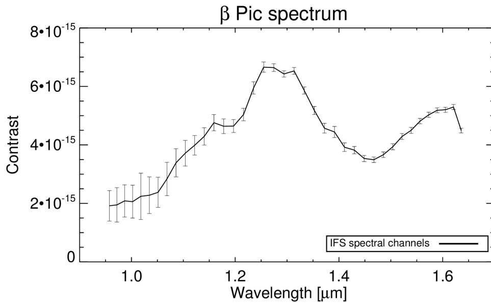
Figure 4.12: Spectrum of \beta Pic b, extracted with KLIP reduction.
