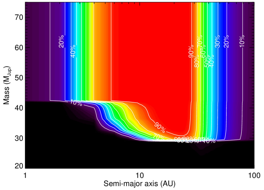
Figure 5.14: Result of QMESS simulation which explores the probability of detection in the parameter space of mass vs semi-major axis for the planet around HD 142 A.
