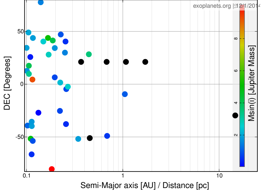
Figure 5.1: Sample of long period objects selected from exoplanet.org database. The criteria of selection (declination, angular separation) are detailed in the text.
