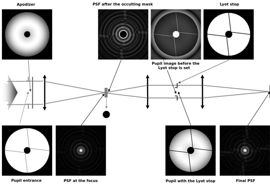
Figure 1.10: Principles of the ALC with a VLT pupil. Image adapted from Guerri et al. (2009).
