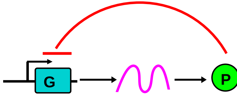
Figure 1.6: A minimal genetic network. In this circuit, the gene synthesizes mRNA which produces the associated protein. The proteins represses the transcription of its own gene, which forms a negative feedback loop. This minimal genetic network actually exists in the nature, such as Hes1, Hes7, involved in somite segmentation, or LexA which is the SOS regulon in E.Coli .
