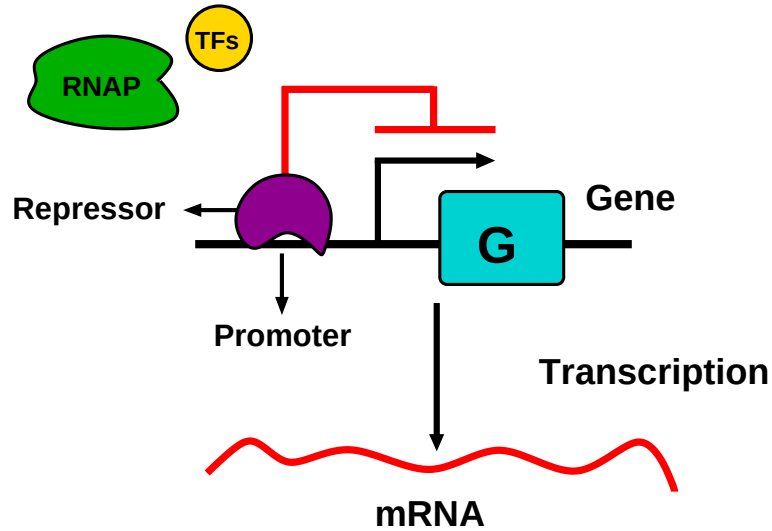
Figure 1.5: Transcription regulation. The promoter is a particular region near the beginning of a gene. The binding of a repressor to the promoter prevents attachment of RNAPs and TFs so that it represses the transcription rate.
