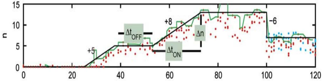
Figure 1.16: Transcriptional bursting in individual cells. The mRNA transcripts tagged by fluorescence proteins are counted in real time t in single cell. The experimental result directly demonstrated that the gene is transcribed during short periods of activity of duration \Delta t_{ON} interspersed by silent intervals of duration \Delta t_{OFF} . The averages of these two periods are \langle \Delta t_{ON} \rangle \approx 6 min and \langle \Delta t_{OFF} \rangle \approx 37 min. Therefore, the autonomous dynamics of gene activity has a time scale comparable to that of other important processes. Figure taken from [85].
