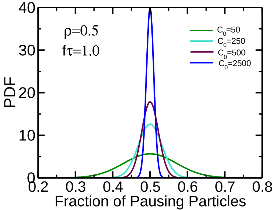
Figure 4.4: Probability density function (PDF) P(\tilde{n}) of configuration with the fraction of paused particle between \tilde{n} and \tilde{n} + d\tilde{n} . When the size of TASEP model increases gradually, this Normal distribution becomes narrower and narrower and the maximum value of PDF is approaching to infinite. In the limit of infinite size, PDF turns to be the Dirac function.
