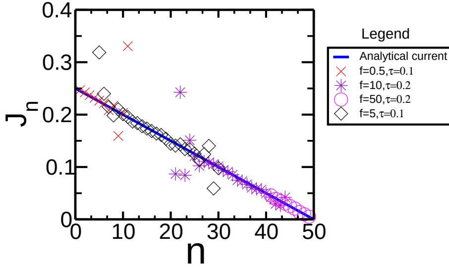
Figure 4.5: Contribution to current as a function of the number of paused particles in the finite-size TASEP model. The blue solid curve is obtained by Eq. (4.11). Different colored symbols represent numerical estimations for fixed parameters values N = 100, \rho = 0.5 . Certain estimations deviate from the curve because of statistical fluctuations, since these configurations have lower probabilities. Therefore, the expression (4.11) predicts well the contribution to current of configurations.
