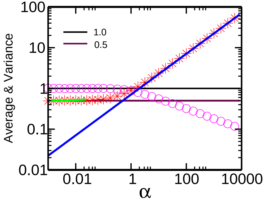
Figure 1.15: Comparison of numerical average and fluctuation level of stochastic dimerization with theoretical predictions of the cumulant expansion. Red stars (resp., magenta circles) represent the numerical average concentration \langle x \rangle (resp., variance-to-mean ratio \sqrt{\Delta_{xx}}/\langle x \rangle ) in the stochastic dimerization process. The variance to mean ratio is approaching to unity for \alpha \ll 1 , which indicates that the system dynamics is driven by protein production following a Poisson process. The blue (green) curve is the steady state predicted by cumulant expansion for the limit case where \alpha \gg 1 (resp., \alpha \ll 1 ). Both limits agree well with numerical simulations.
