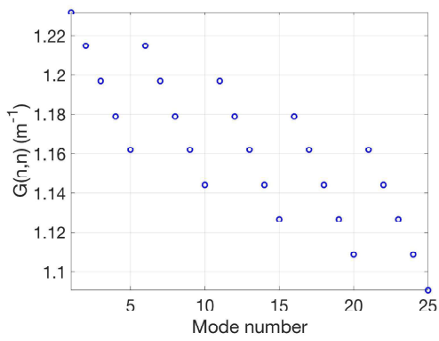
(c) Gain per mode
