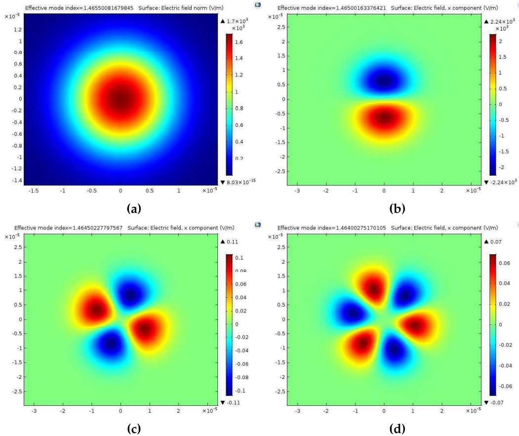
Figure 3.2: Fundamental and high order modes obtained by Comsol Multi-physics mode solver: (a) LP_{01} (b) LP_{11} (c) LP_{21} (c) LP_{31}
