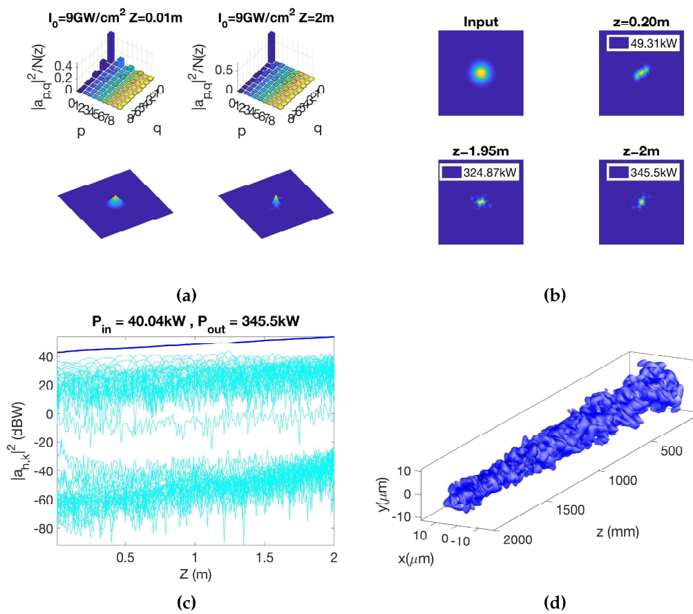
Figure 6.10: Kerr, gain and disorder without saturation: (a) Fraction power of modes at beginning and end of fiber length (b) Intensity profile plot of input and output guided modes (c) Fractional power evolution of modes (d) Iso-intensity plot across fiber length
