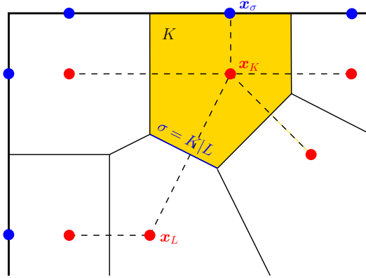
Figure 3.1 – Illustration of an admissible mesh as in Definition 6.
