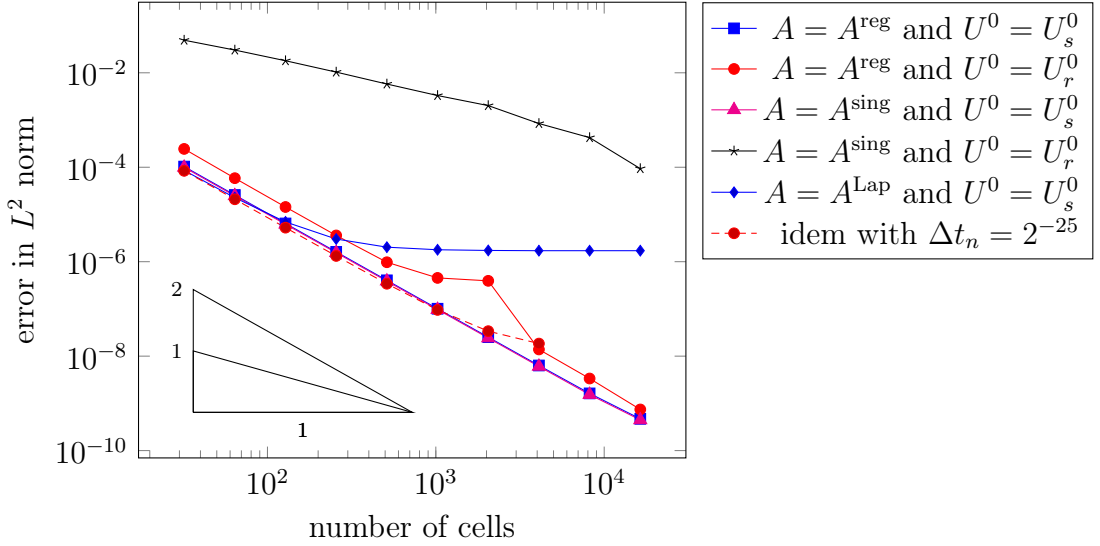
Figure 5.2 – Error with respect to reference solution.
