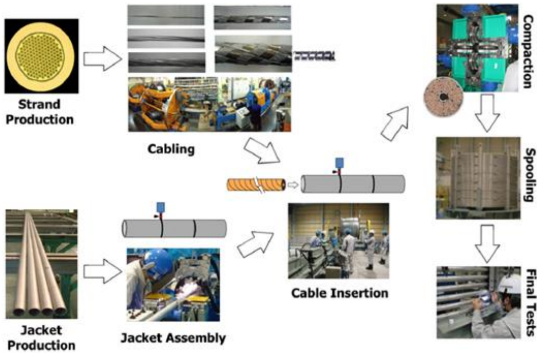
Figure I.2.10. Main steps of ITER CICC manufacture (Devred 2014).
