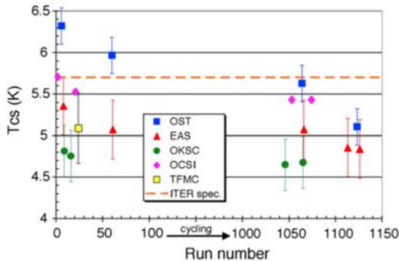
Figure I.2.14. T_{cs} degradation due to EM cycling in a typical SULTAN test (Ciazynski 2007).
