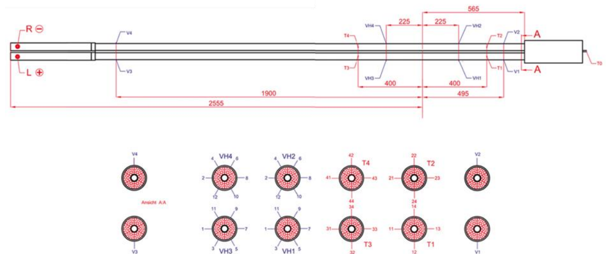
Figure I.2.12 reports a schematic drawing of the SULTAN samples and probes installed on the conductors jacket.
