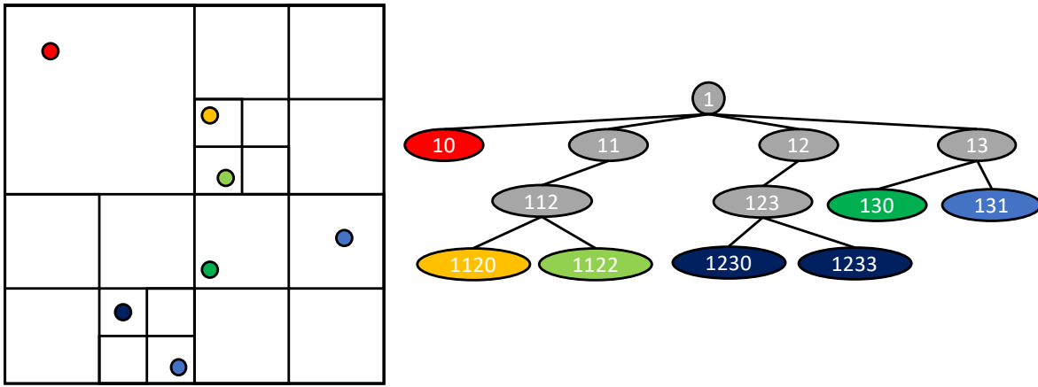
Figure 7.5: This figure represents the particles and the space division used to create the quadtree on the right. The nodes are the intermediate divisions and the leaves are the particles' data.
