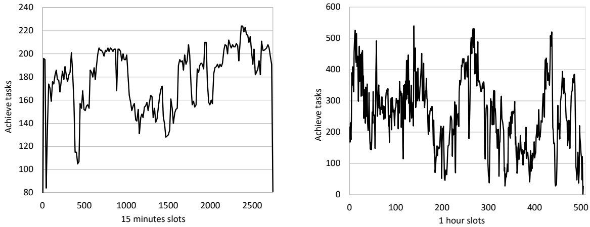
(a) Best-Effort tasks per 15" slots for L(2,27) . (b) Best-Effort tasks per 1 hour slots for L(2,28) .
