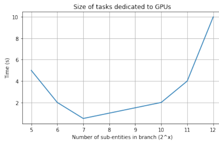
Figure 7.13: The task balancing between the CPU and GPU is determined by the depth in which the CPU will generate the tasks. If it is too high the GPU will have too much work to handle and to low the tasks will be too small to use the potential of the GPU.
