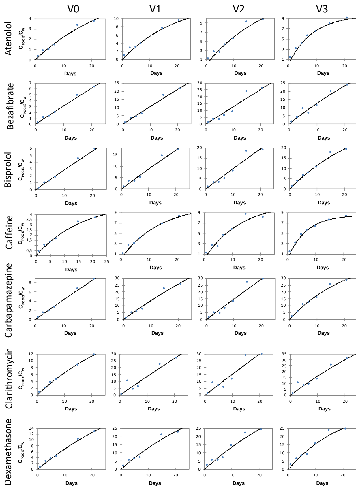
Figure A.1: C_{POCIS}/C_w versus deployment time (days).
