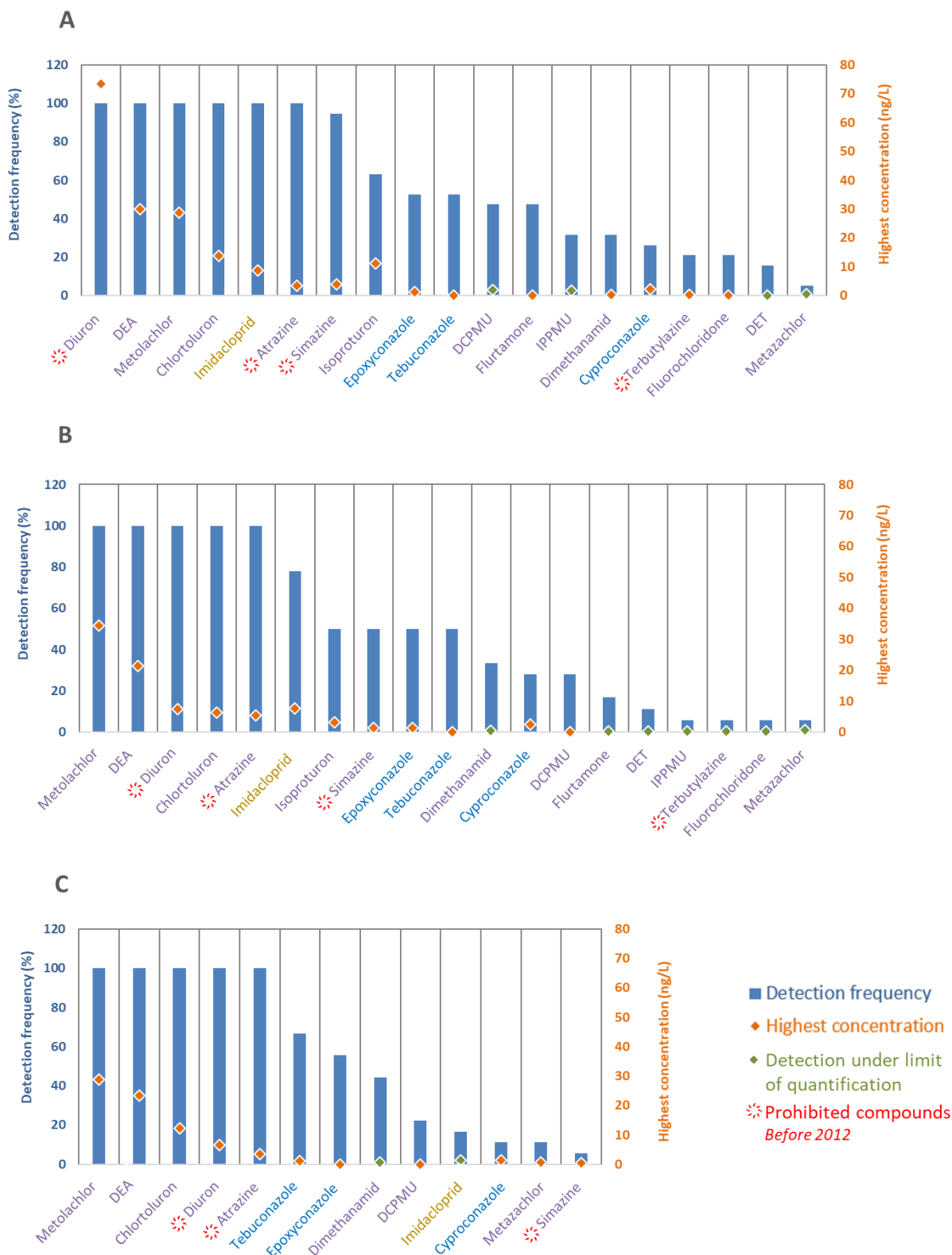
Figure V.6: Pesticide detection frequencies and highest concentrations determined with POCIS at the Aixette watershed in 2016 (POCIS exposures=19): A: Aixette Upstream, B: Aixette Downstream and C: Arthonnet. Herbicides, fungicides and insecticides are in purple, blue and yellow, respectively.
