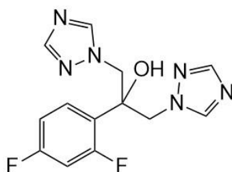
Figure 76: Structure de fluconazole
