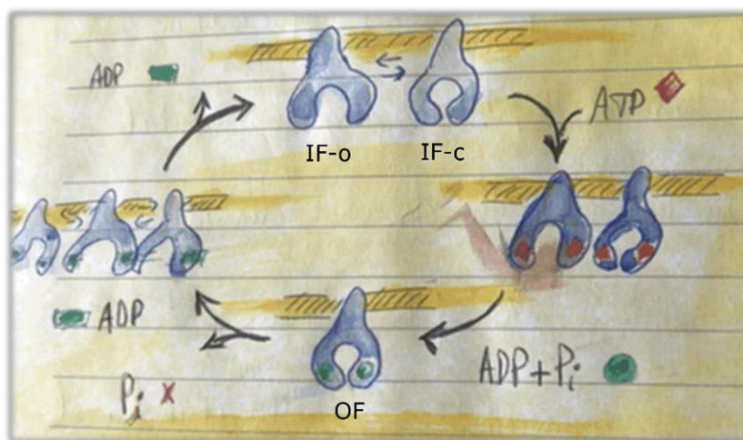
Scheme 1: Representation of the transporter cycle of ABC transporters involving ATP hydrolysis and the large conformational changes between IF-o, IF-c and OF conformations.
