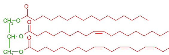
Figure 7: Representation of a triglyceride. The glycerol moiety and the N-acyl chains are depicted in green and red, respectively.
