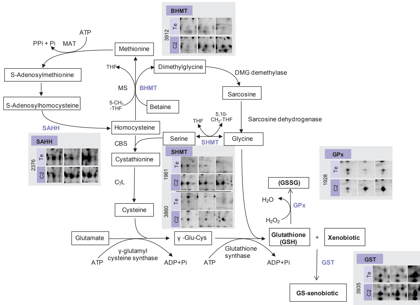
Figure 7: Hypothetic cycle implying BHMT, SHMT, SAHH GST and GPx. For each identified protein, images of the spots are shown in T29Te vs T29C2 condition. CBS, cystathionine beta synthase; CγL, cystathionine gamma lyase; MS, methionine synthase; BHMT, betaine homocysteine methyltransferase; SHMT, serine hydroxymethyltransferase; GST, glutathione S transferase; GPx, glutathione peroxidase
