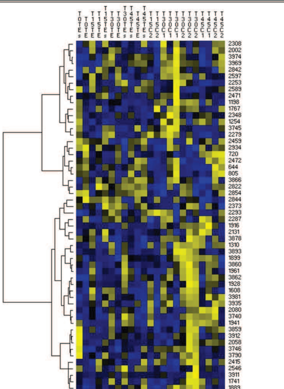
Figure 4: Heat map based on the normalised integrated volumes given by the Progenesis sameSpot software for spots found significantly deregulated in this study (see methods for parameters used in PermutMatrix).
