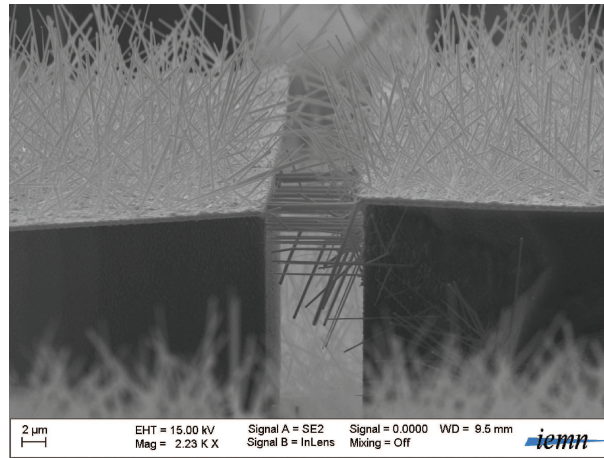
Figure 3.1: Silicon nanowires grown between walls parallel to the surface. Gap between walls: 8 \mu\text{m} .
