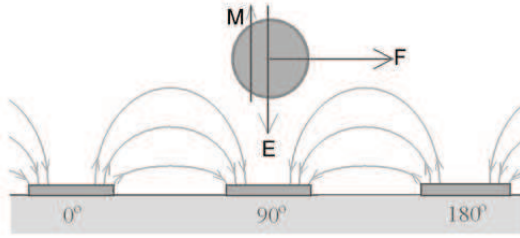
Figure 3.11: Traveling dielectrophoresis. An array of interdigitated electrodes creates a traveling field. On the object will be acting trapping ( F_{trap} ) and propagating ( F_{prop} ) forces.
