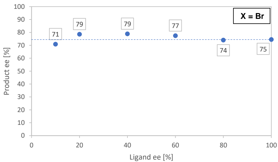
Figure 56: Hyperpositive NLE of the Br-NBE catalysed addition of ZnEt 2 to benzaldehyde.
