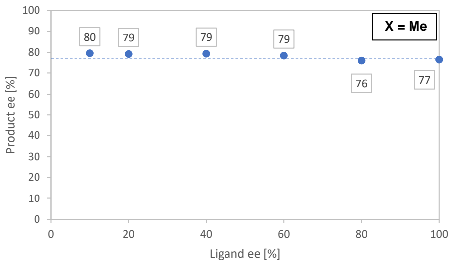
Figure 55: Hyperpositive NLE of the Me-NBE catalysed addition of ZnEt 2 to benzaldehyde.
