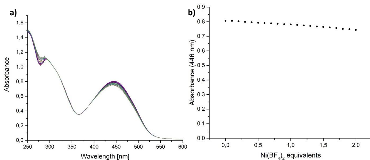
Figure 127: a) UV-vis titration of ligand 26 ( 5,74 \cdot 10^{-5} M in THF) with \text{Ni}(\text{BF}_4)_2 -aliquots (0.1 equiv. each), b) evolution of the absorbance at 446 nm over the course of the titration.
