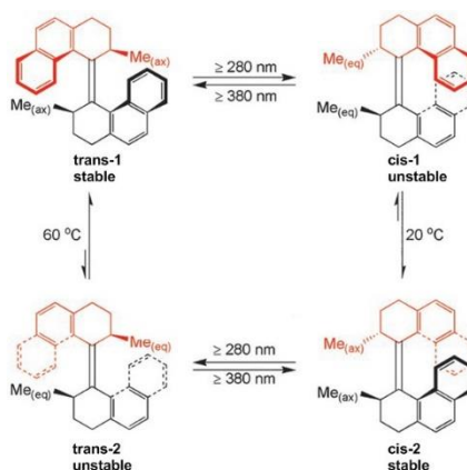
Fig. 20 Operation of an unidirectional molecular rotor.
