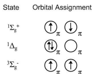
Fig. 2.5 Representation of singlet and triplet oxygen states.
