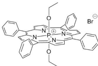
18, [P(TPP)(OEt) 2 ] + Br -
