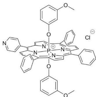
23, [P(MPyP)(OPhOMe) 2 ] + Cl -
