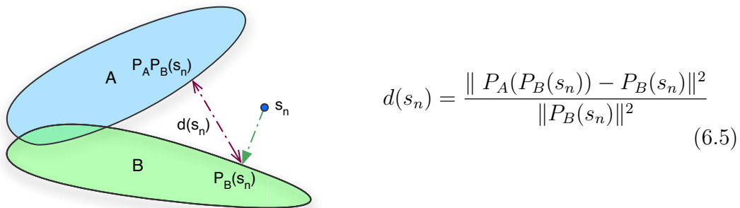
FIGURE 6.8 Distance interensembles
