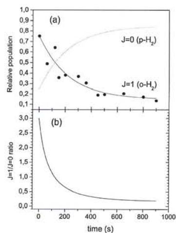
Fig. 2 Time evolution of the J -selected relative populations of 0.75 ML \text{H}_2 on porous ASW with 0.012 ML of co-adsorbed \text{O}_2 ; (a) o\text{-H}_2 ( J = 1 ) (full circles). Single exponential fitted function f(t) = A + (1 - A)\exp(-t/\tau) of the o\text{-H}_2 ( J = 1 ) population (full line); time evolution given by [1 - f(t)] for the p\text{-H}_2 ( J = 0 ) population (dashed line) (b) time evolution of the J = 1/J = 0 ( o/p ratio) given by f(t)/[1 - f(t)] . Parameters A and \tau are given in Table 1.
