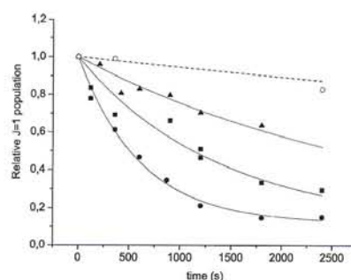
Fig. 3 Time evolution of the relative p\text{-D}_2 ( J = 1 ) population measured by REMPI and after thermal desorption from ASW; 0.75 ML \text{D}_2 with 0.012 ML \text{O}_2 (full circles); 0.25 ML \text{D}_2 with 0.012 ML \text{O}_2 (full squares); 0.75 ML \text{D}_2 with 0.001 ML \text{O}_2 (full triangles); 0.75 ML \text{D}_2 , with 0 ML \text{O}_2 (open circles). Full lines are fitted functions f(t) = A + (1 - A)\exp(-t/\tau) ; dotted line is a linear fit. Parameters A and \tau are given in Table 1.
